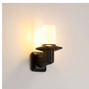
MK-W02193 POWER:6W IP RATING:IP65 SIZE:252*160*115MM INPUT:AC85-265V
